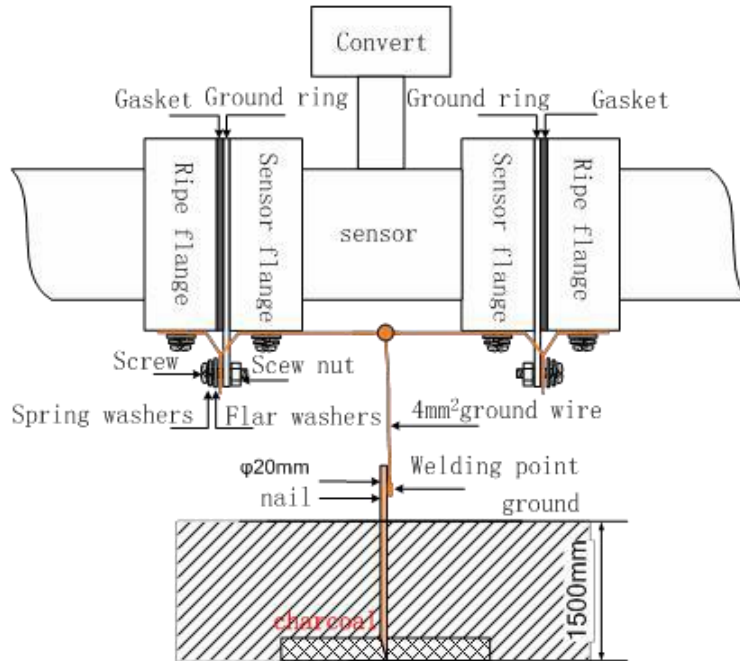
Fig.4.4(f) Grounding
