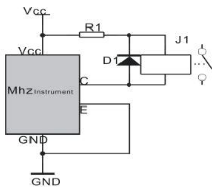
Conventional relay
